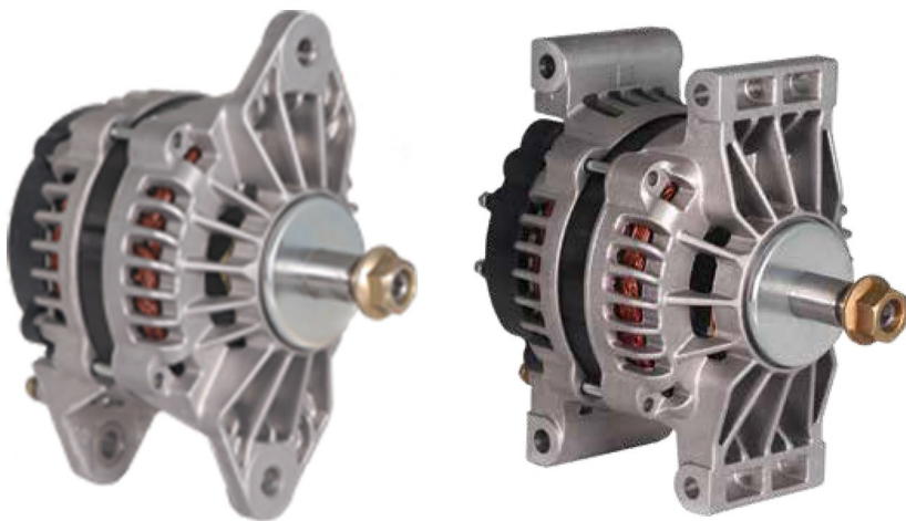
24SI Alternator (Replaces 22SI) 12 Volts • 160 AMPS • 1 Year/Unlimited Mile Warranty
